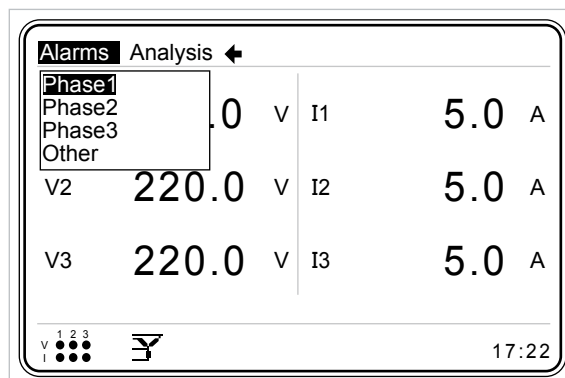
Figure 3-90 Alarms Menu
