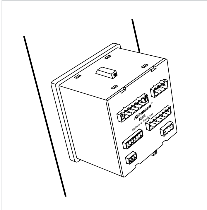
Figure 2-2 Fixing KLEA to the panel
