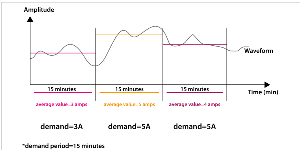
Figure 3-71 Demand Example
