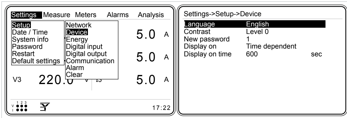
Figure 3-19 Device Menu
