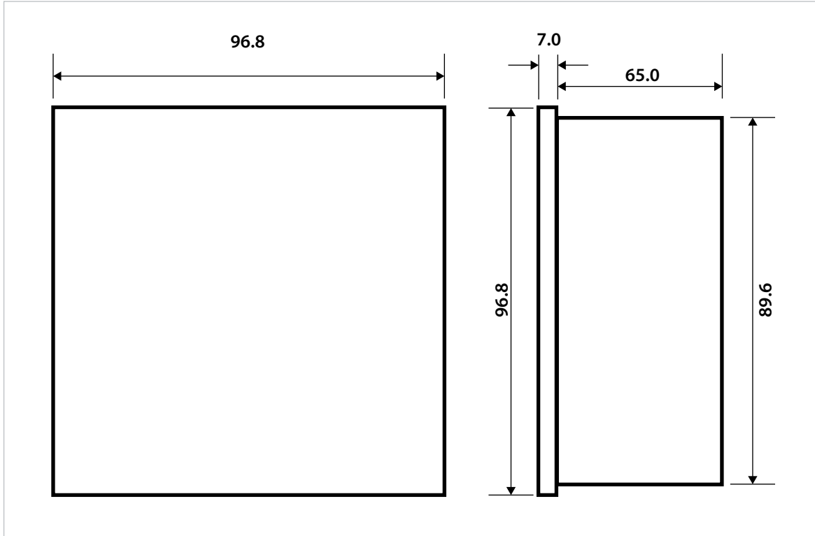
Figure 2-9 Dimensions
